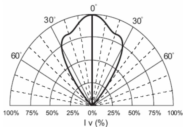
Radiation Diagram
