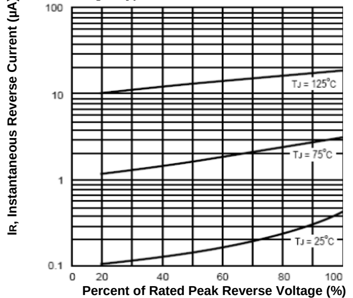
Fig.4-Typical Reverse Characteristics
