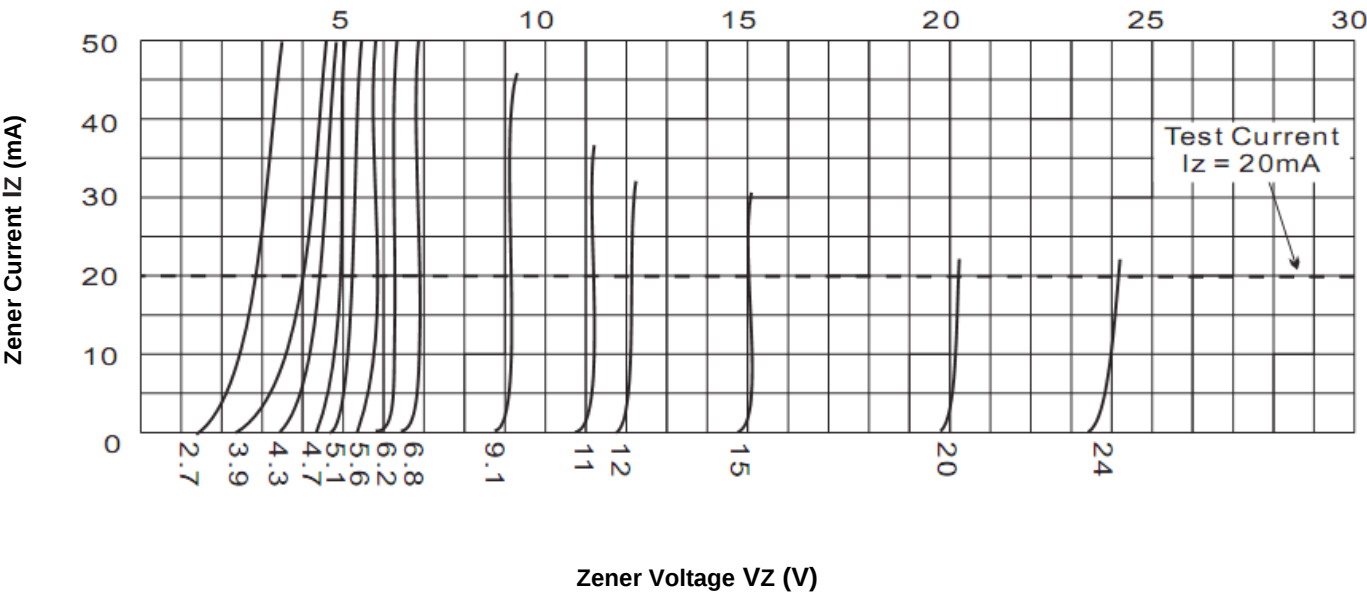
Fig.2-Breakdown Characteristics
