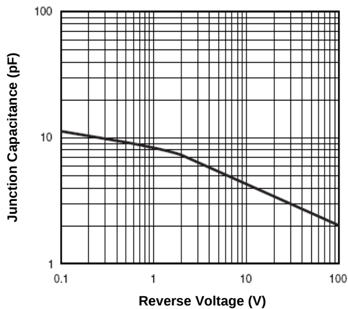
Fig.5-Typical Junction Capacitance
